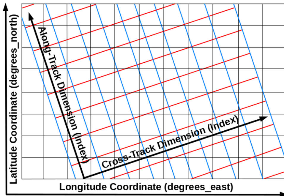
Figure 2 The horizontal dimensions (along_track and cross_track) and coordinates (latitude and longitude) for a swath product. In some products the horizontal dimensions and coordinates can be one and the same (e.g., latitude and longitude).
